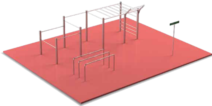
Street Workout Park Queens Dimension: Park 7 x 2 m, Dip-Barren 2.35 x 1.05 m
