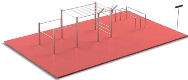
Street Workout Park Brooklyn Dimension: Park 5.1 x 2 m, Dip-Barren 2.35 x 1.05 m
